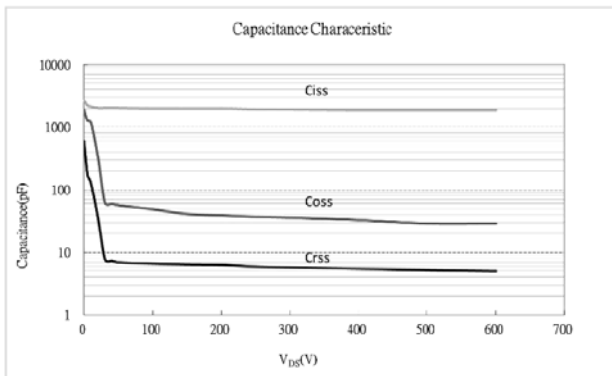
Figure 5: Typical Ciss, Coss, Crss, vs. Vds @ TJ=25 °C
