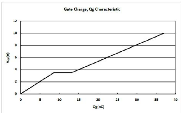
Figure 3: Typical VGS vs. Qg @ Vds=400 V TJ=25 °C
