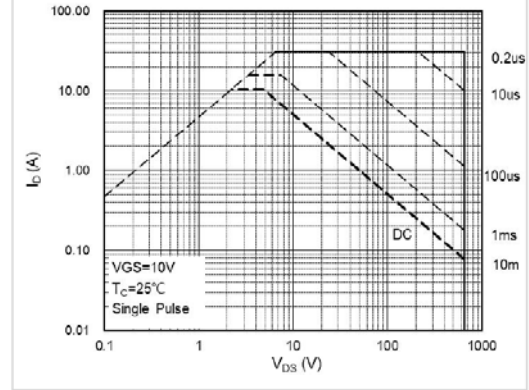
Figure 8: Ids vs. Vds SOA @ Tc = 25 °C
