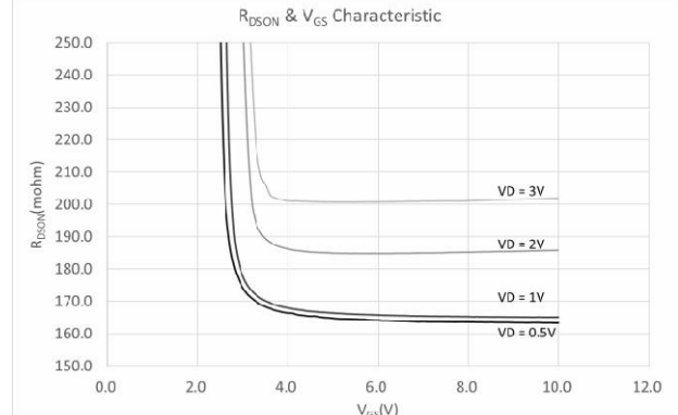
Figure 4: RDSON vs. VGS Characteristic @ TJ = 25 °C
