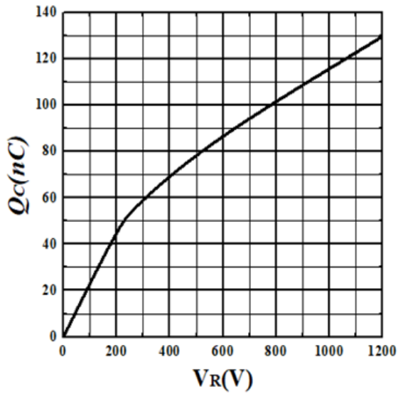
Figure 7. Total Capacitance Charge vs. Reverse Voltage
