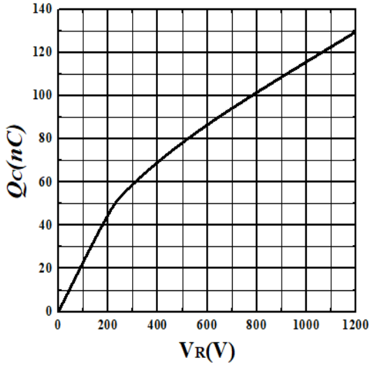
Figure 7. Total Capacitance Charge vs. Reverse Voltage
