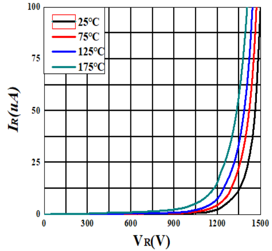
Figure 2. Reverse Characteristics
