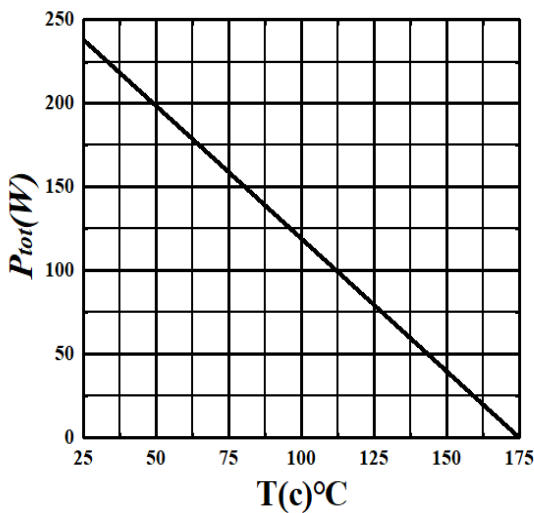
Figure 5. Power Derating
