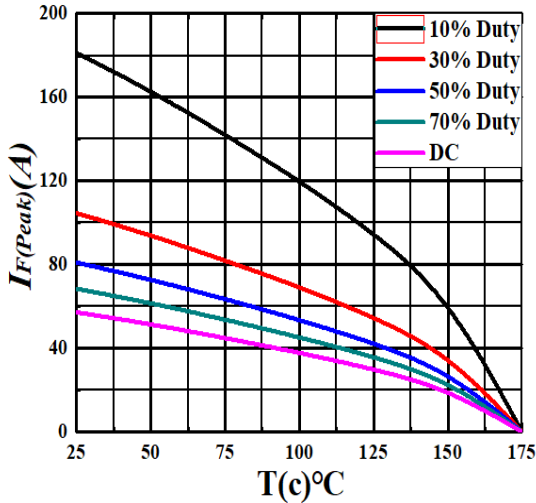
Figure 3. Current Derating
