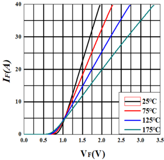
Figure 1. Forward Characteristics
