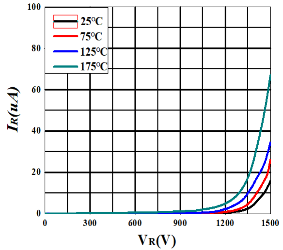
Figure 2. Reverse Characteristics
