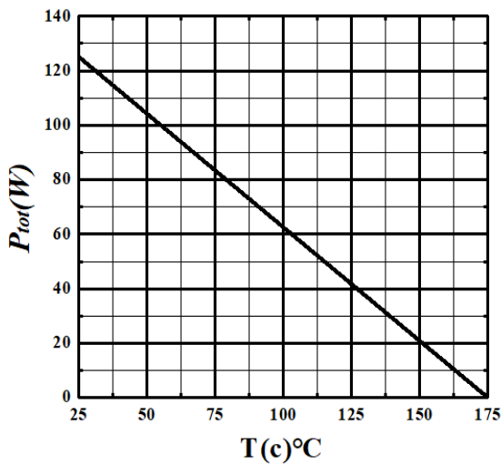
Figure 5. Power Derating
