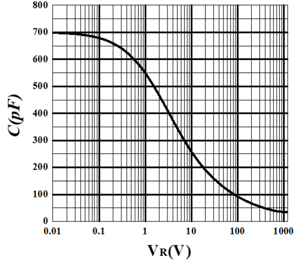
Figure 4. Capacitance vs. Reverse Voltage
