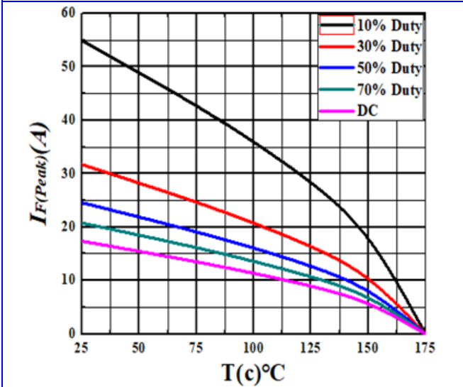
Figure 3. Current Derating
