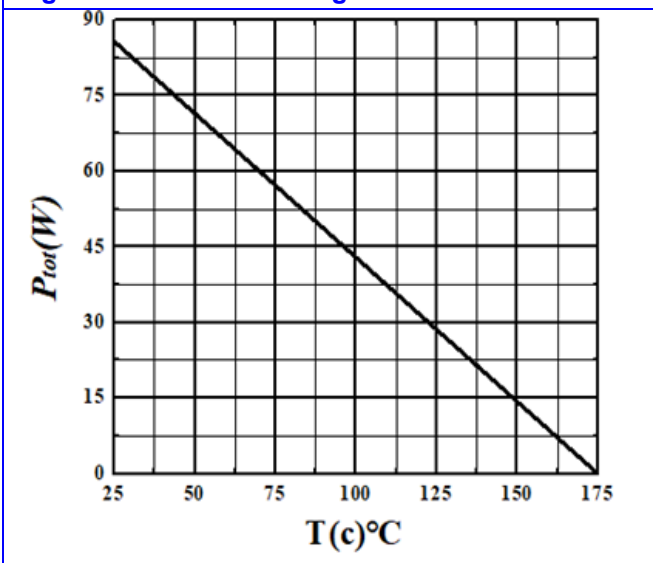
Figure 5. Power Derating
