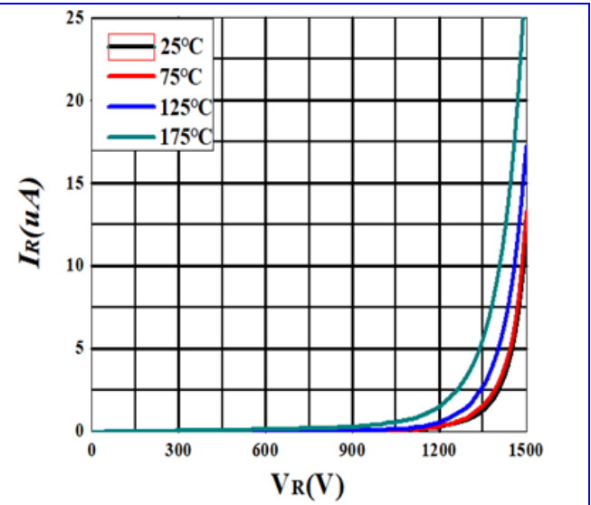
Figure 2. Reverse Characteristics
