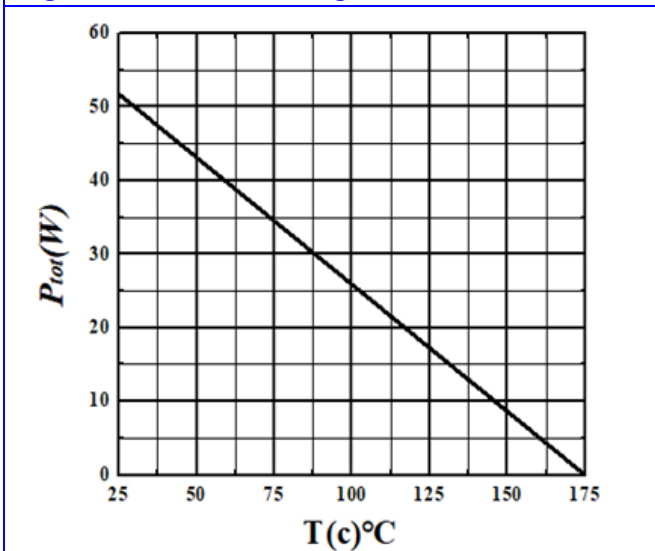
Figure 5. Power Derating
