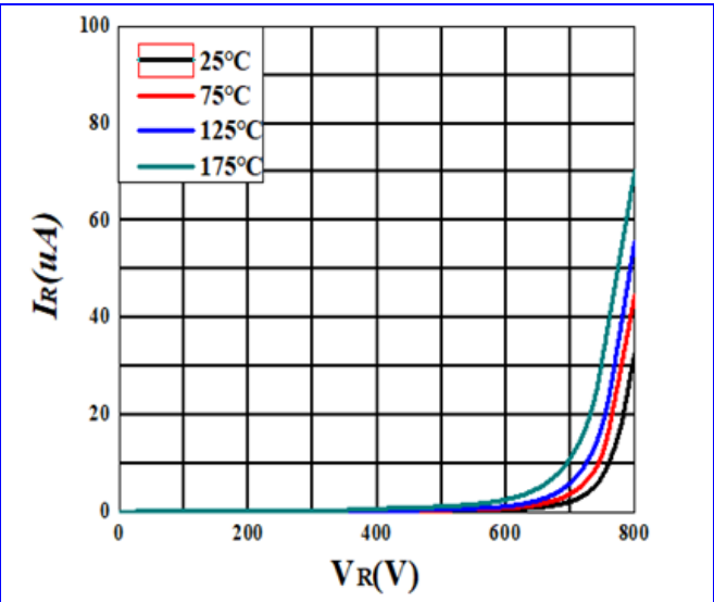
Figure 2. Reverse Characteristics
