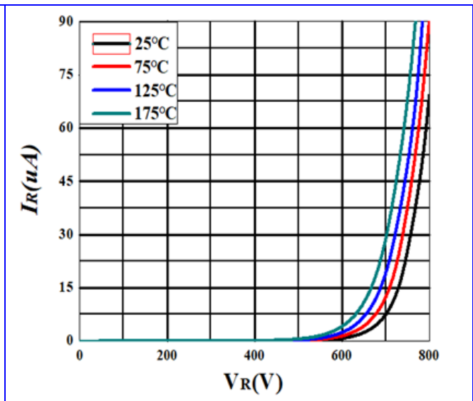
Figure 2. Reverse Characteristics
