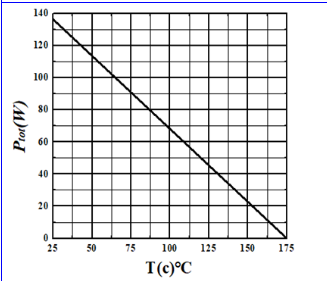
Figure 5. Power Derating
