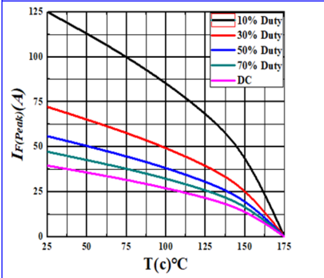
Figure 3. Current Derating
