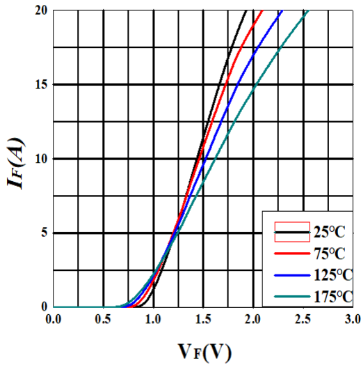
Figure 1. Forward Characteristics
