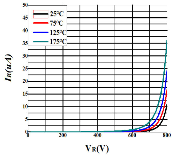
Figure 2. Reverse Characteristics
