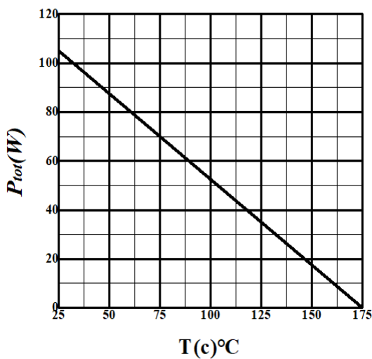
Figure 5. Power Derating
